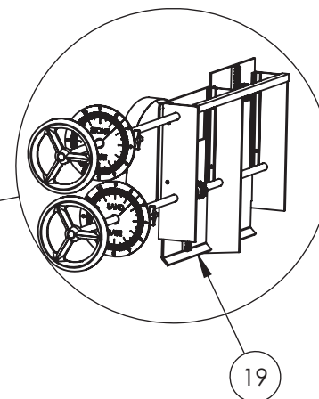
METERING GATE ASSEMBLY (COMPLETE) BAY-LYNX PART# MG100-ASM-1
